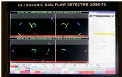
Display mode: B-Scan for one channel
